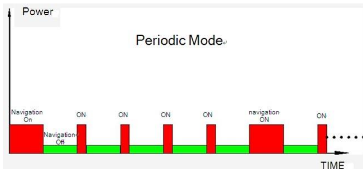
Figure 5 Periodic Mode
