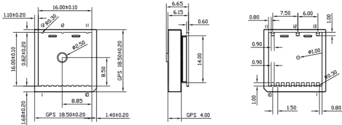
Figure 3 CG37 mechanical dimensions (Unit: mm)
