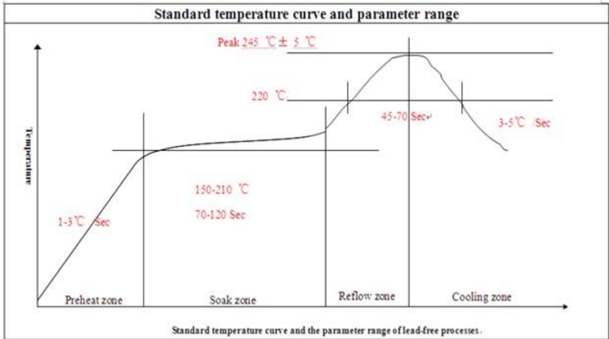
Figure 10 The Ramp-Soak-Spike reflow profile of CG37
