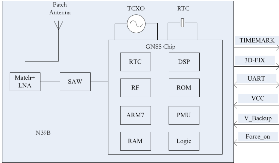
Figure 1 CG37 functional diagram
