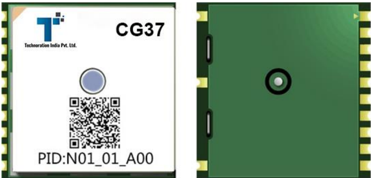
Figure 9 Top and Bottom View of CG37
