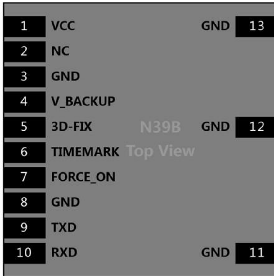
Figure 2 CG37 pin out diagram (Top view)
